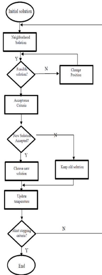
Figure 1. The simulated annealing algorithm
