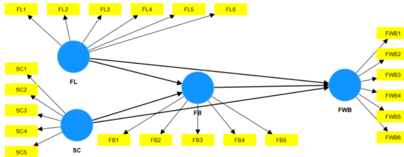
Gambar 2. Diagram Path
