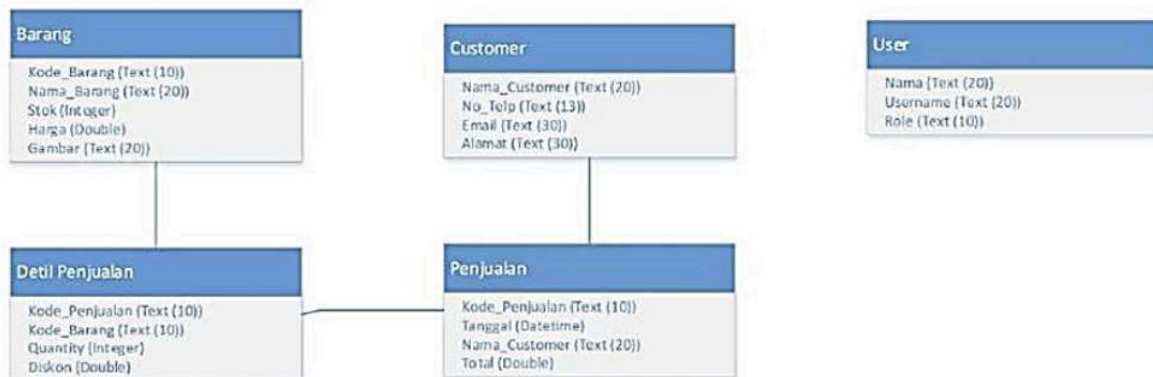
Gambar 4. Class diagram Tiara Handicraft
