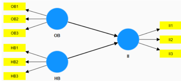
Gambar 2. Diagram Path
