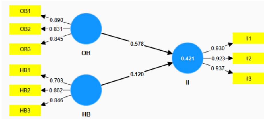
Gambar 2. Outer Model
