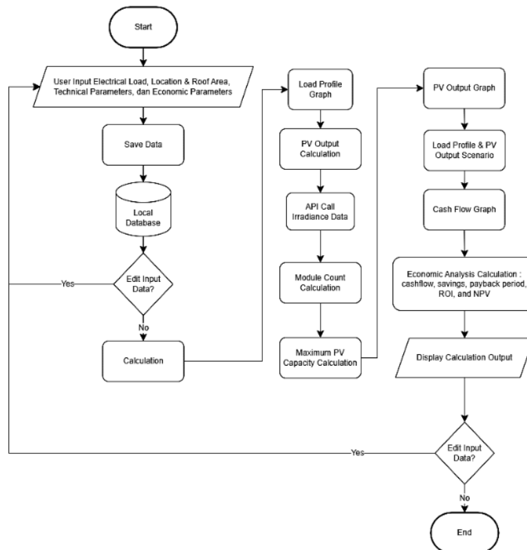
Figure 2. Flowchart of KawanSurya
