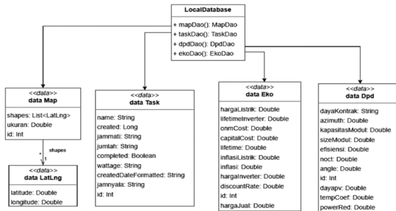
Figure 4. KawanSurya database scheme
