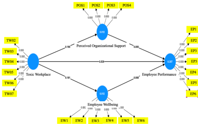
Figure 2. Inner Model Results Source: primary data processing
