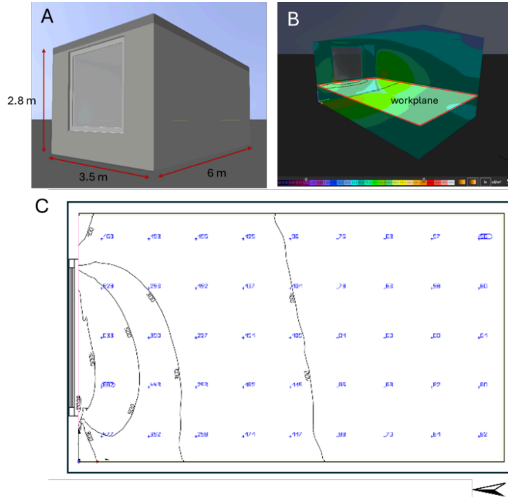
Figure 1. The model of the building created in DIALux Evo (a), the luminance on workplane (b), and the position of the sensor points (c).
