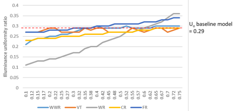
Figure 4. Illuminance uniformity ratio of the model with various variable values.
