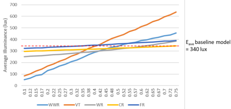
Figure 3. Average illuminance of the model with various variable values.
