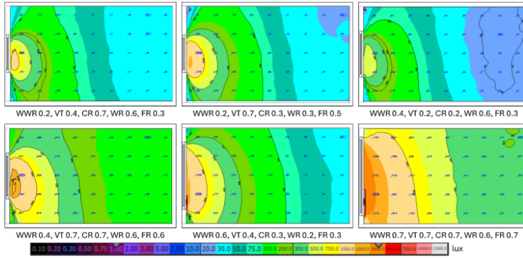
Figure 5. Average illuminance of the model with various variable values.
