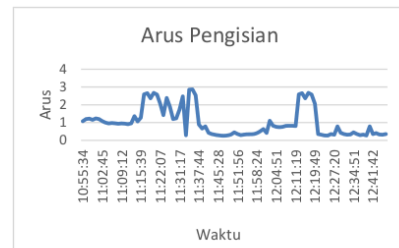
Gambar 14. Grafik Arus Pengisian 21 November 2022
