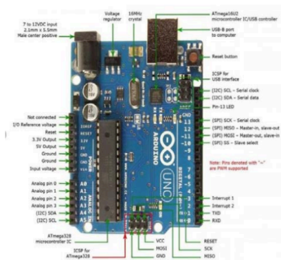
Gambar 2. Board Arduino Atmega328
