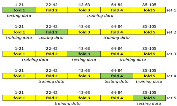
Figure 2 Five-Fold Cross-Validation Model
