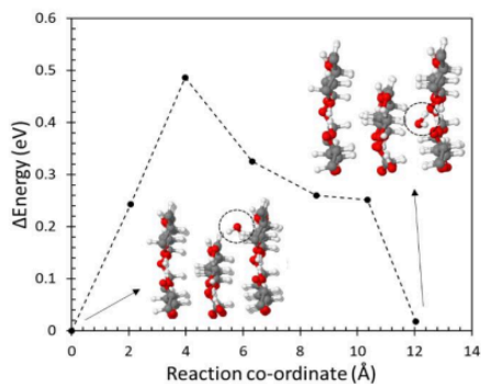
FIGURE 3. Minimum energy path of a water molecule absorption on the [010] surface of the cellulose model. The water molecule is shown inside the dotted circle.
