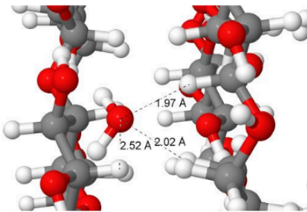
FIGURE 7. Water molecule on the [11] surface of the cellulose with the distances between its oxygen atom and the nearest hydrogen atoms of cellulose chains.
