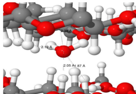
FIGURE 8. Water molecule in the [10] subsurface of the cellulose with the distances between its oxygen atom and the nearest hydrogen atoms of cellulose chains.
