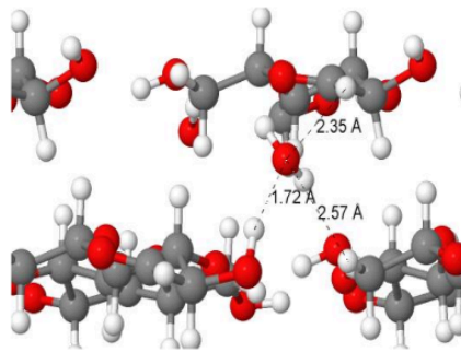
FIGURE 6. Water molecule on the [10] surface of the cellulose with the distances between its oxygen atom and the nearest hydrogen atoms of cellulose chains.
